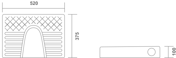
SQUATTING - 1715 L 520 | W 375 | H 100 mm MRP: 1150/-
