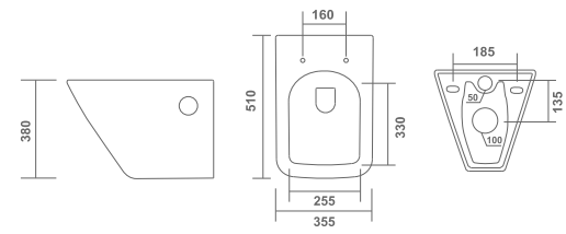
POOL - 1104 L 510 | W 355 | H 380 mm MRP: 6130/-
