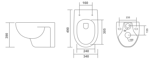
JETTA - 1106 L 490 | W 340 | H 390 mm MRP: 4980/-
