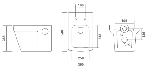
STELLA - 1103 L 540 | W 360 | H 385 mm MRP: 6130/-
