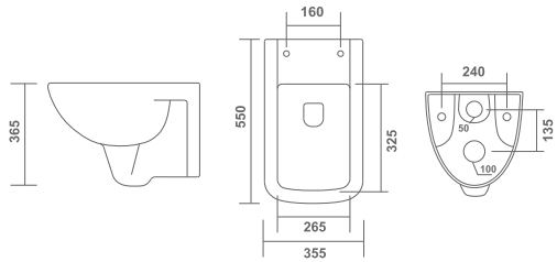
OPAL - 1101 L 550 | W 355 | H 365 mm MRP: 5120/-
